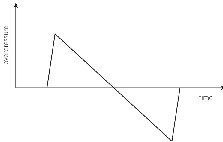
FIGURE 2. AN N-WAVE
